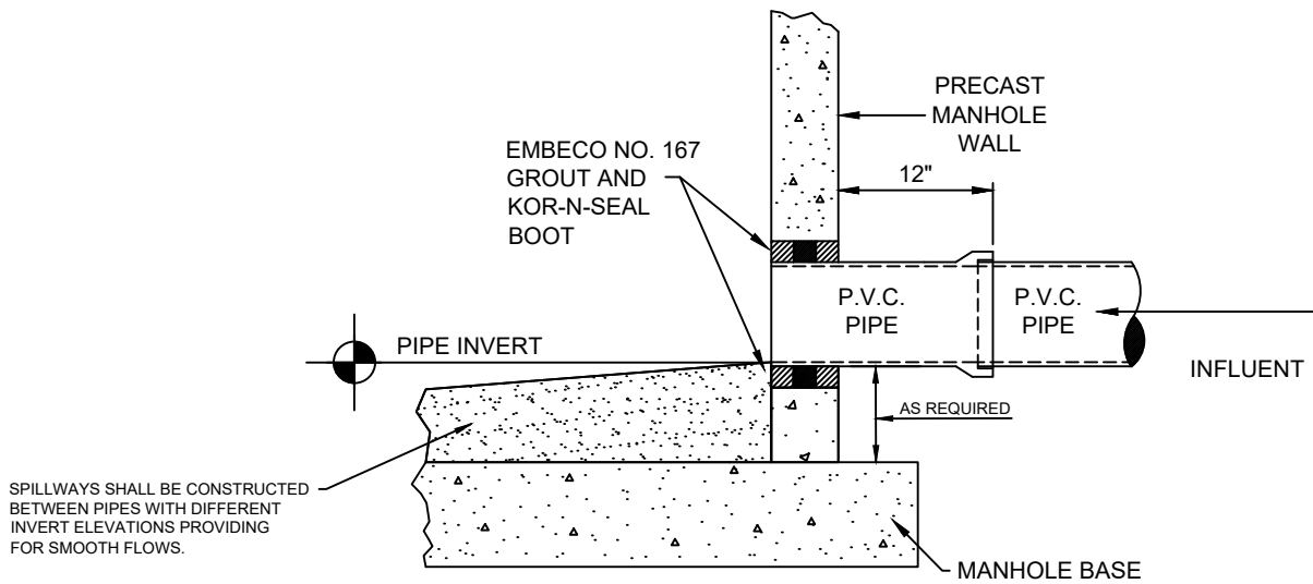
INFLUENT CONNECTION
