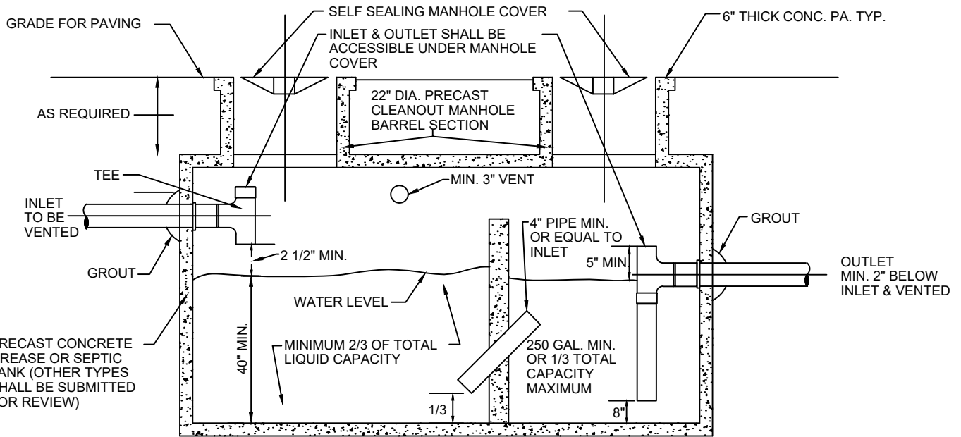
SECTION
